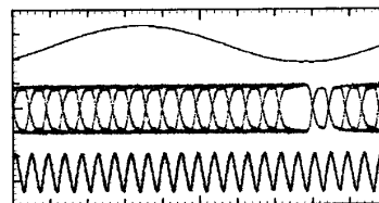
Fig. 10. TX input clock, transmitted frame, and RX recovered clock at 1.5 GBd.
