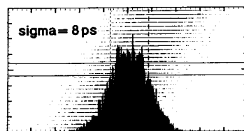
Fig. 11. Phase jitter histogram of RX recovered clock at 1.5 GBd.
