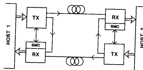
Fig. 1. Block diagram of full-duplex link built from two chip-set pairs.
